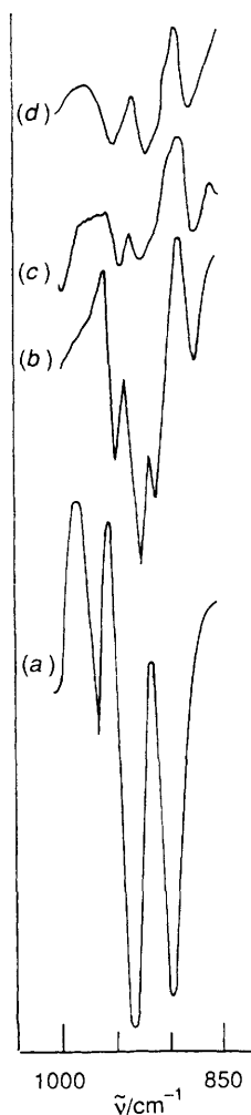
Fig. 1 Infrared spectra of (a) [MoO 2 (pacda) 2 ], (b) [MoO(pacda) 3 ]BF 4 , (c) [Mo(PPh 3 )(pacda) 3 ]BF 4 and (d) [Mo(acda)(pacda) 3 ]BF 4 showing gradual abstraction of oxygen atoms from the cis -MoO 2 2+ precursor
