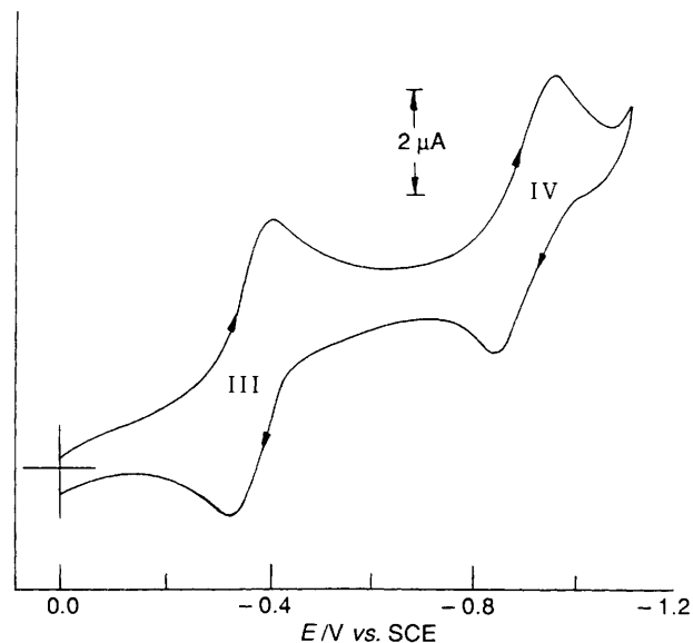
Fig. 3 Cyclic voltammogram of [Mo(PPH_3)(pacda)_3]BF_4 ( 1.2 \times 10^{-3} \text{ mol dm}^{-3} ) in dmf at an HMDE. Supporting electrolyte, 0.1 \text{ mol dm}^{-3} NEt_4ClO_4 ; scan rate, 50 \text{ mV s}^{-1}
